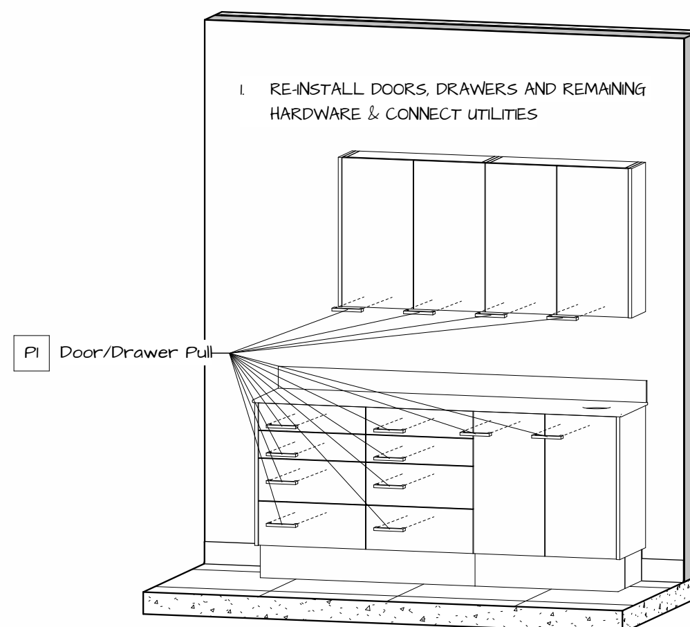
2.4 Install Hardware
