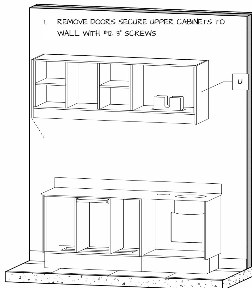
2.3 Install Upper Cabinets
