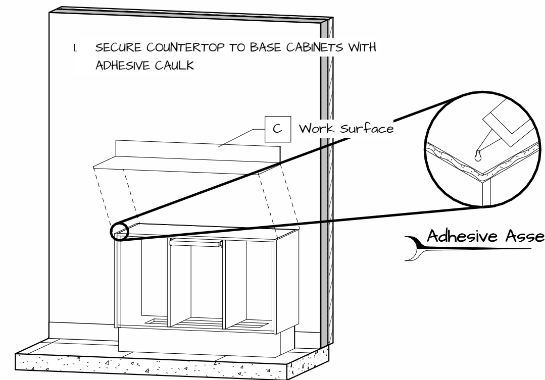
2.2 Install CounterTop
