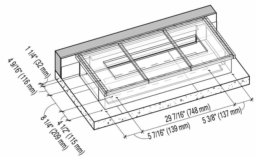
2 Utilities Access
